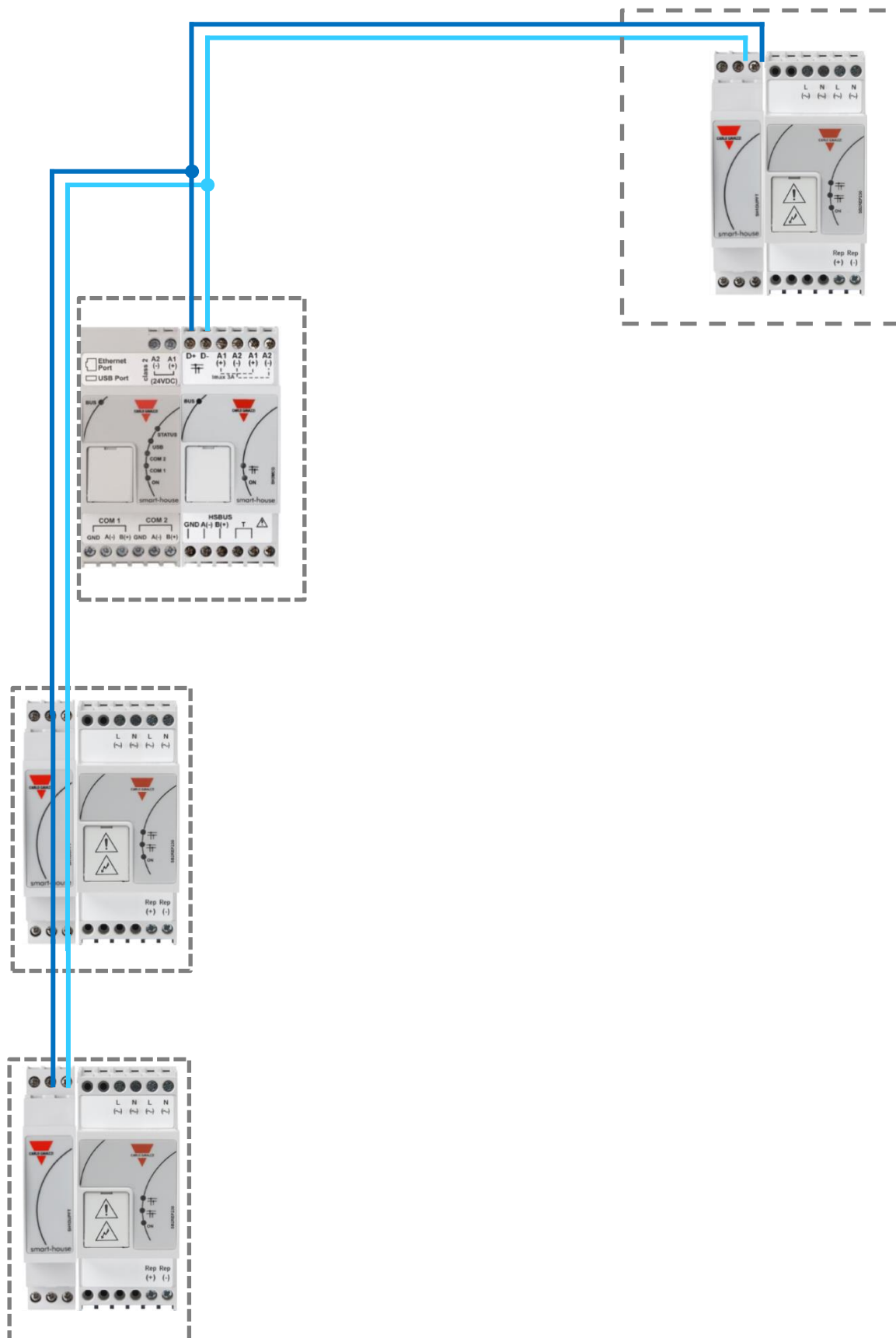
Installation des Sx2WEB-Systems
