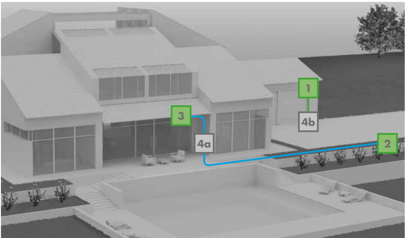
1 SHSP90L PIR sensor with integrated luxmeter
